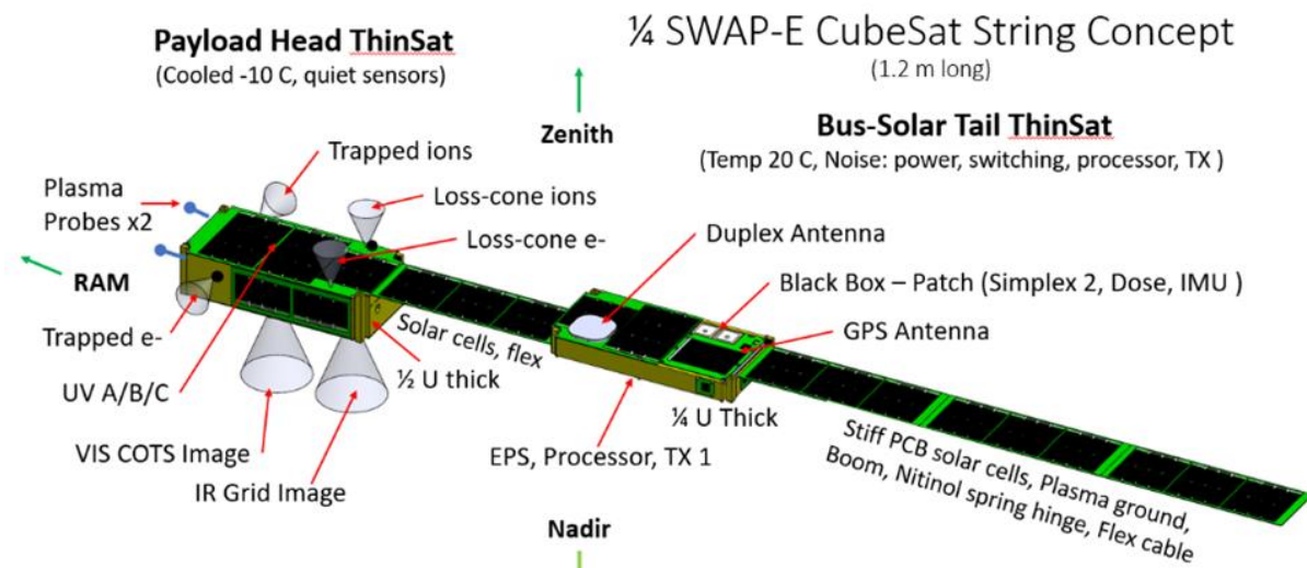
Figure 7 SWAP-E constellation layout for each of the four constellation CubeSats released from a standard 2U by 3U launcher unfold into a 1.2 m string as shown by two ThinSats and four Solar Array panels. The Larger ThinSat (5cm thick) contains the sensitive and passively cooled SW sensors while the ThinSat Bus (2.5 cm thick) contains all the relatively noisy spacecraft system functions of power, transmitters, flight processor, and solar arrays. A shielded electrical flat flex cable connects all of the foldouts and two ThinSats.
