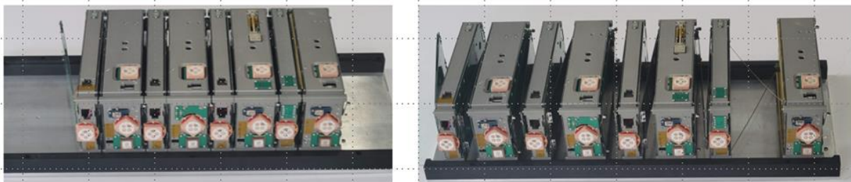
Figure 8 Final Flight SWAP-E four Satellite constellation in 6U Launch configuration (Left side) and illustrates how the four satellite strings unfold as they leave the 6U canister. Note the VLF two wire antennas fold out naturally with the last string unfolding. Also note all of the 12 EyeStar patch antennas.
